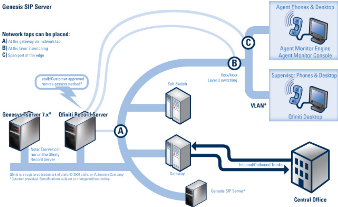
Figure 5: Genesys LAN Tapping Positions
